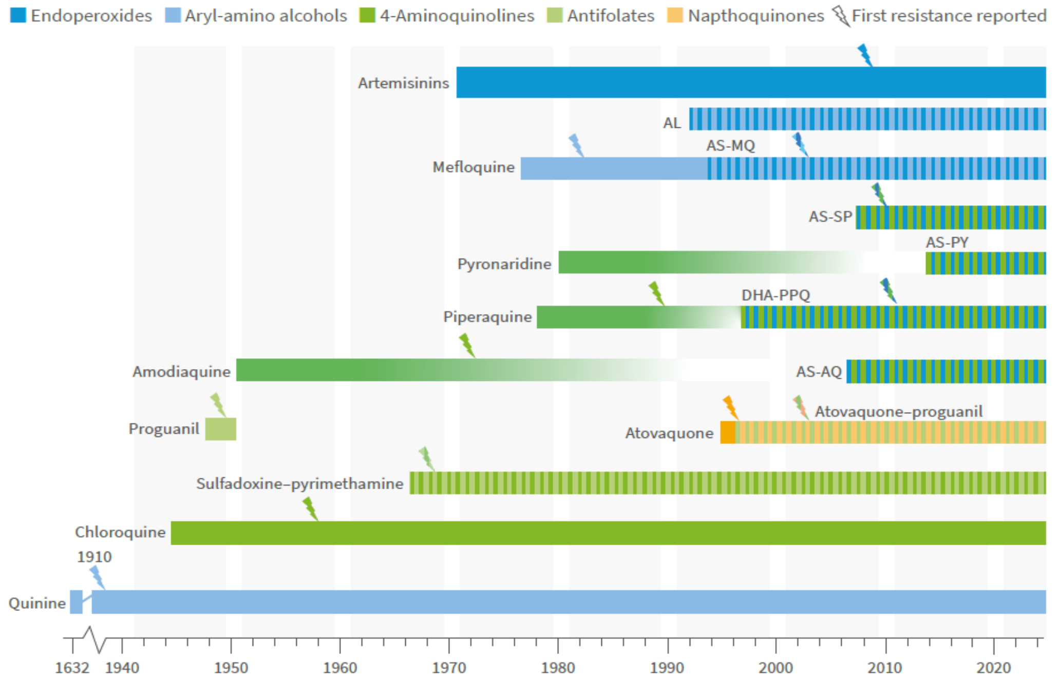
Fig. 7.1. History of introduction of principal antimalarials and of first emergence of resistance in the field Source: Adapted from Blasco, Leroy and Fidock (123).
